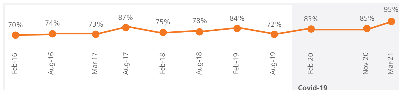
Figure 5. MCQ Pass-Rates
