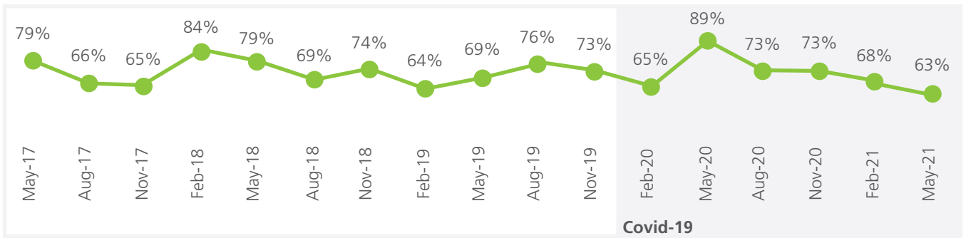
Figure 7. PWC Pass-Rates
