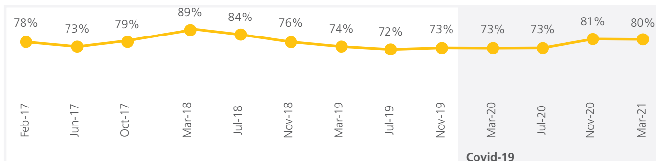
Figure 8. SP Pass-Rates
